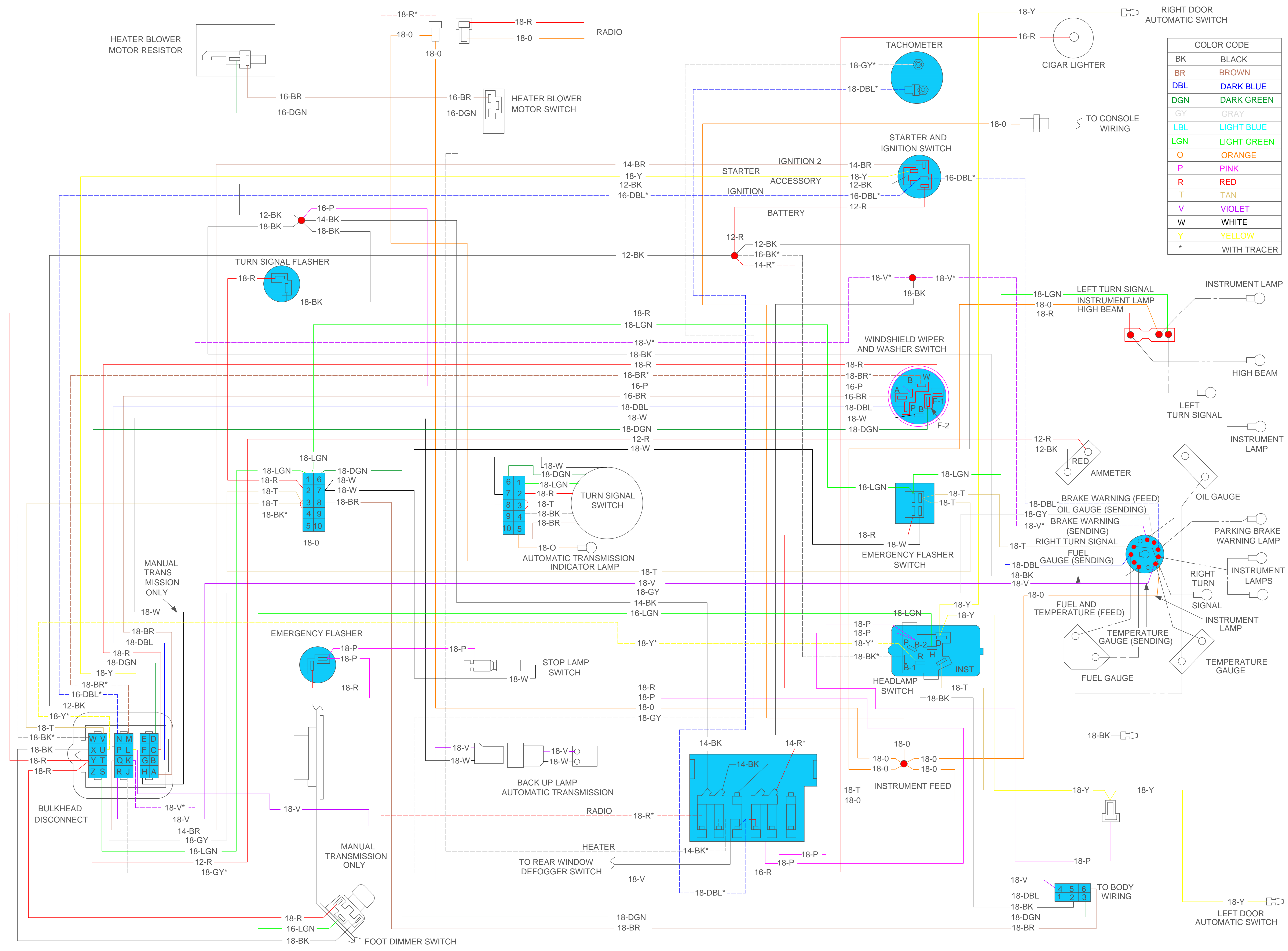
INSTRUMENT PANEL WIRING - BARRACUDA 1967
